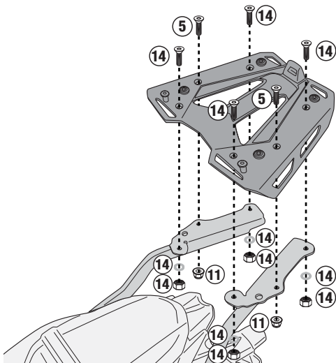
M6M PLATE
